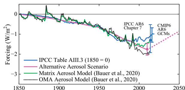
Figure 18. Aerosol forcing relative to 1850 from IPCC AR6, an alternative aerosol scenario [151] two aerosol model scenarios of Bauer et al. [154].
