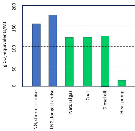
FIGURE 3 Full lifecycle greenhouse gas footprint for LNG for both short and long cruises compared with coal used domestically, diesel oil used domestically, natural gas used domestically, and electric-power ground-source heat pump powered by the average European electric grid. The LNG values are the means for the three types of tankers that burn LNG for fuel. Methane emissions are converted to carbon-dioxide equivalents using GWP 20 . Note that values are expressed per unit of heat energy for each fuel for delivery to an electric generation plant. This does not include methane emissions from urban distribution systems that deliver to buildings for heat. Emissions for LNG and natural gas used domestically would both increase substantially for this use of gas. See text. GWP 20 , 20-year global warming potential; LNG, liquefied natural gas.
